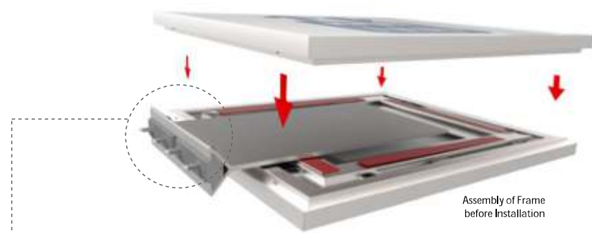
2 FLEX READY MADE (PROJECTED) SECTION DETAILS ISOMETRIC VIEW SCALE: NTS
