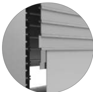
TRIPOST CONNECTORS Tri-Post TLB50 and TLSLO Joining Alliance Insert and face Profiles with TLPAN for stability purpose - see drawing below
