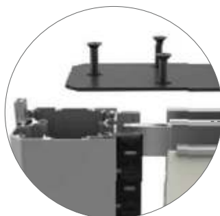
TRILINE - Combined with Splendid and Alliances Components ( TLOPV & TLCLJ) Synthetic Lock to the Tri-Post TLTMSP80 with Synthetic Cover Plate.
